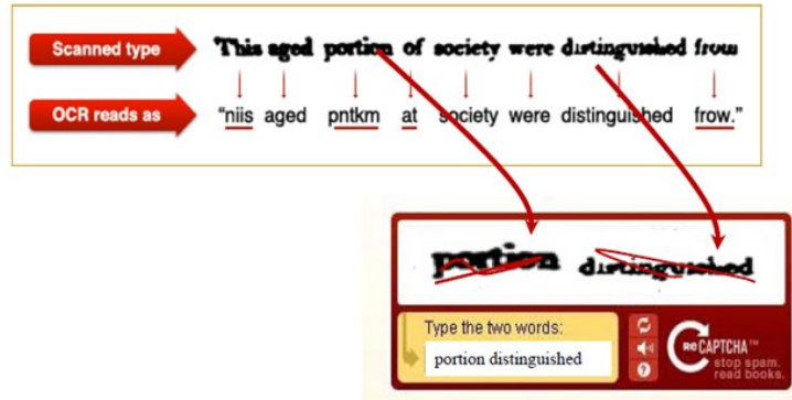
Figure 5.4. Diagram explaining how reCAPTCHA works according to https://www.google.com/recaptcha
