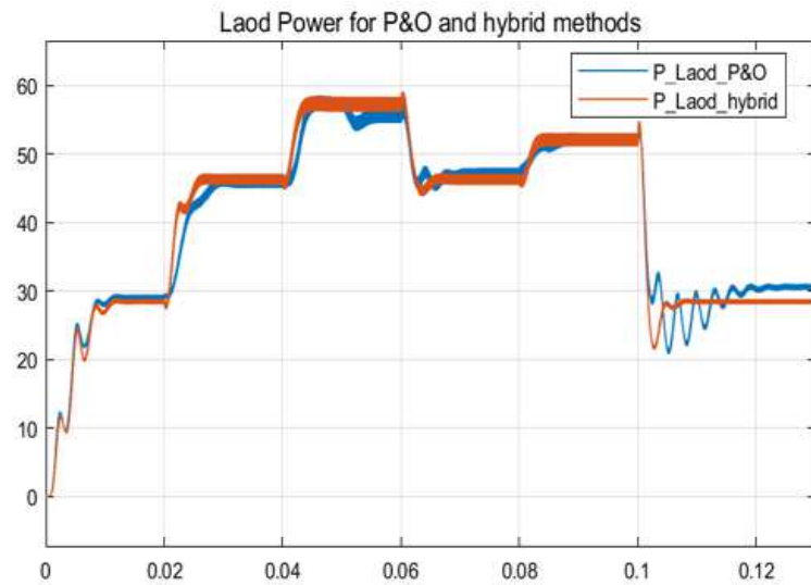
Figure 10. Load power for hybrid and P&O (a) MPPT under variable solar irradiation and temperature.
