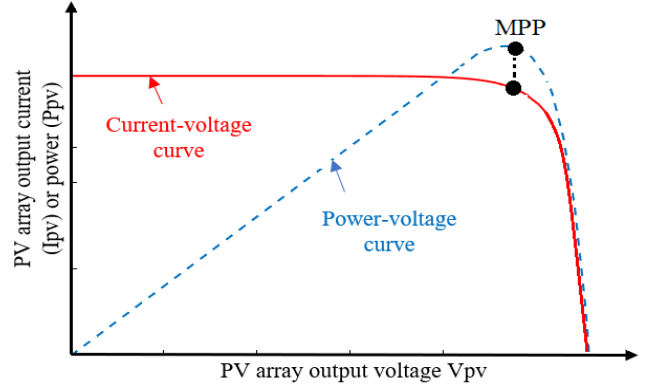
Figure 2. Curve of the current and power at the output of the module PV depending on the output voltage.
