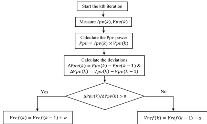
Figure 4. An algorithm of the MPPT perturbation and observation P&O technique proposed by Hua et al. [19].
