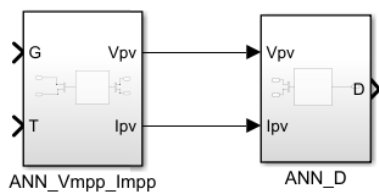
Figure 6. The proposed ANN hybrid controller.
