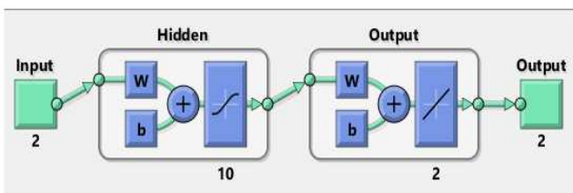
Figure 5. Architecture of the network.
