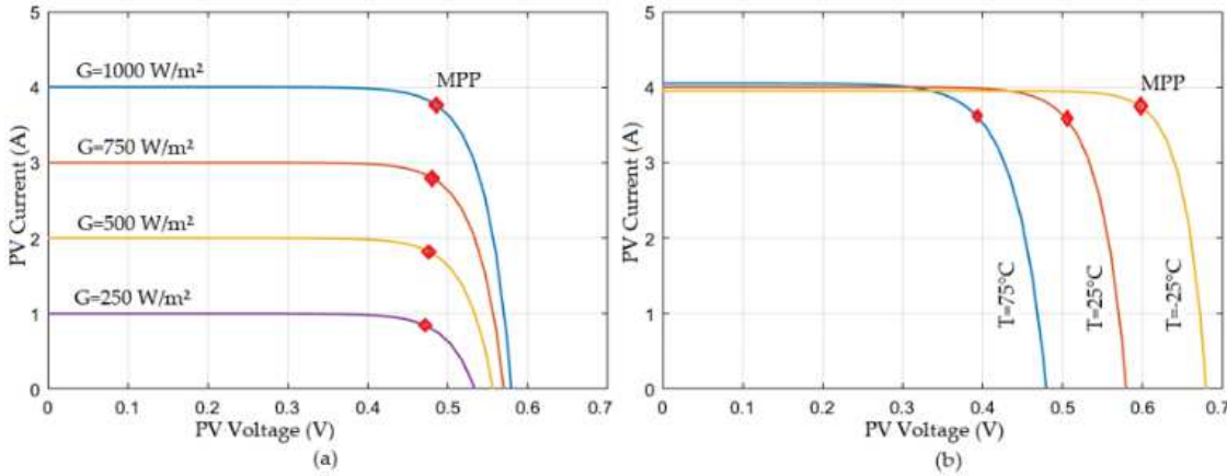
Figure 3. Variation of current and voltage of a PV module depending on the variation of solar irradiation (a) and ambient temperature (b).
