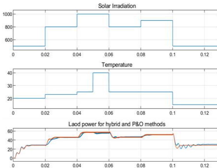
Figure 8. Load input power for P&O and hybrid MPPT controller under variable solar irradiation and temperature.
