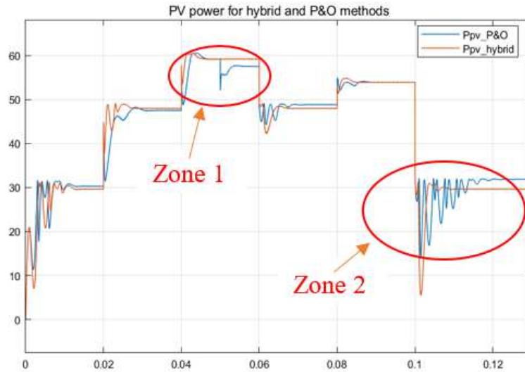
Figure 9. PV power for hybrid and P&O (a) MPPT under variable solar irradiation and temperature.
