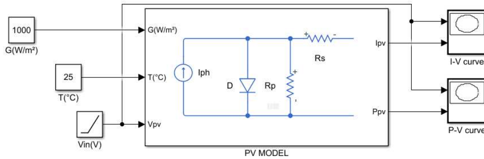
Figure 1. PV model implemented in Matlab/Simulink.
