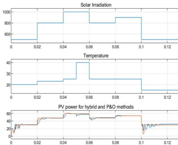
Figure 7. PV array output power P&O and hybrid MPPT controller under variable solar irradiation and temperature.
