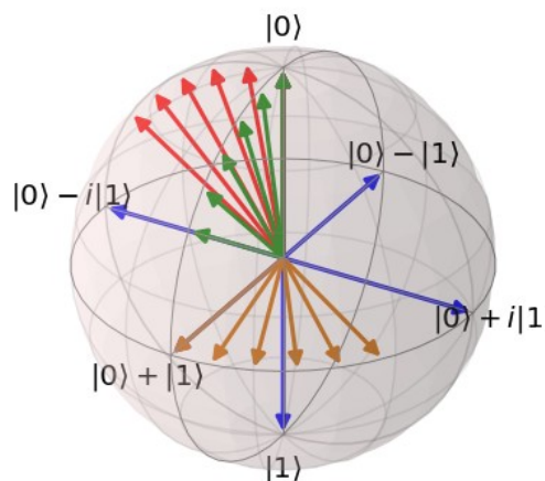
Fig. 3 : Multiple statevectors in a Bloch Sphere.
